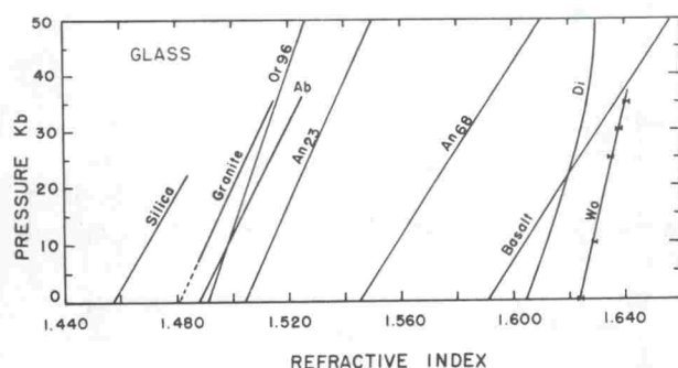
FIG. 4. Pressure-refractive index diagram, showing the change of refractive indices of glasses with pressures. The silica glass was heated to 675°-720°C, but all other glasses were quenched from runs just above the liquidus at high pressure. Wo = \text{CaSiO}_3 glass (present study); Di = diopside glass (Boyd and England, 1963); Basalt = basaltic glass (Cohen, Ito, and Kennedy, 1967); Ab = albite (Boyd and England, 1963); Granite = muscovite granite glass (Huang, 1973); Or 96 = orthoclase glass; An 23 and An 68 = plagioclase glass (Chao and Bell, 1968); and Silica = silica glass (Cohen and Roy, 1965).
