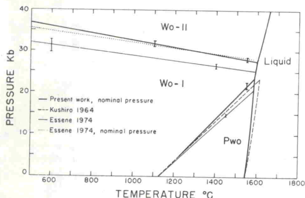
FIG. 2. Phase relations from Figure 1 compared with previous studies by Kushiro (1964) and Essene (1974).
