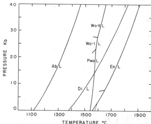
FIG. 3. Experimentally determined melting curves for \text{CaSiO}_3 (Fig. 1), diopside (Boyd and England, 1963), enstatite (Boyd, England, and Davis, 1964) and albite (Boyd and England, 1963).
