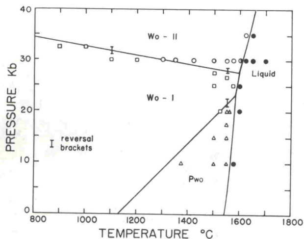
FIG. 1. Experimental results showing the subsolidus and melting relations for \text{CaSiO}_3 . Solid circles denote runs above liquidus; open symbols denote subsolidus runs. The definitive reversal brackets on the subsolidus transitions are shown. Abbreviations: Wo-I, wollastonite I; Wo-II, wollastonite II; Pwo, pseudowollastonite.
